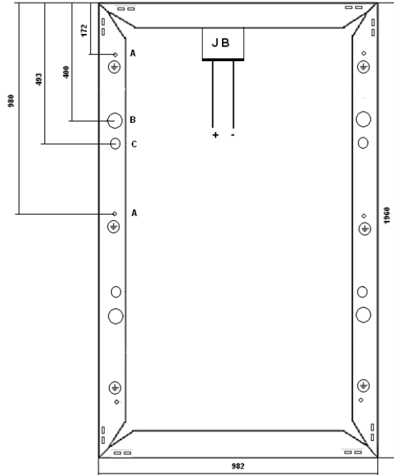
FRAME DRAWING
